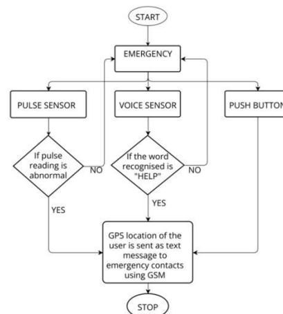
Figure 2: Program Flow Chart
