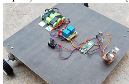
Figure 7: Hardware Kit of obstacle Avoiding Robt Car
