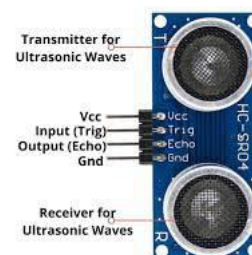
Figure.3: Ultrasonic Sensor
