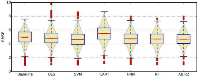
Figure 3: RMSE for each regression algorithm
