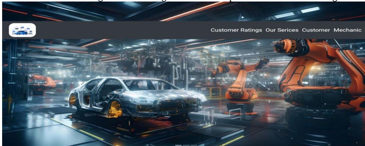
Fig1:Home Page
