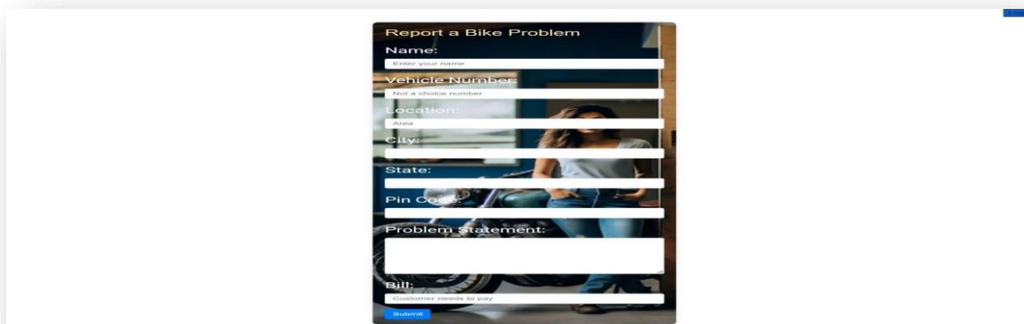
Fig6 : Report page
