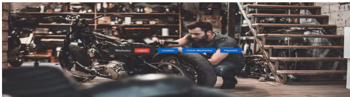
Fig2 :Customer Homepage
