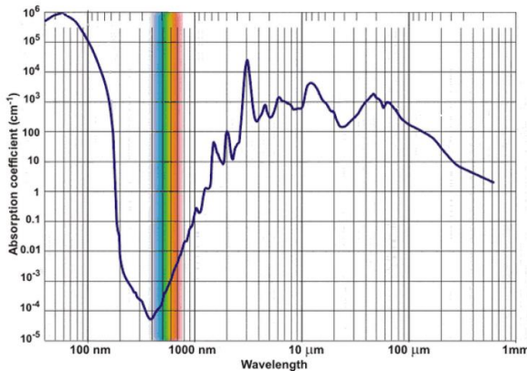
Fig 1. Light absorbtion vs wavelength curve
