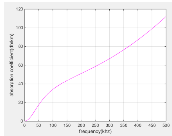
Fig 1. Absorption coefficient versus frequency: Implementation with Thorps' formula
